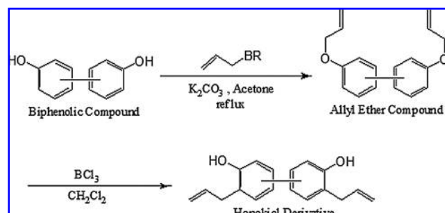
FIG. 8. Synthetic scheme of honokiol and its derivatives. The synthesis of honokiol derivatives by using various bisphenol starting materials via an allylation of the phenolic hydroxyl groups and then the Claisen rearrangement. Various derivatives have different effects on targets and varying toxicity.
